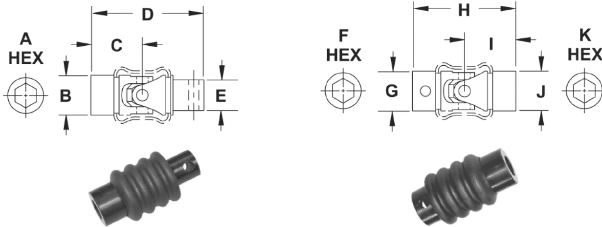
UPPER JOINT
